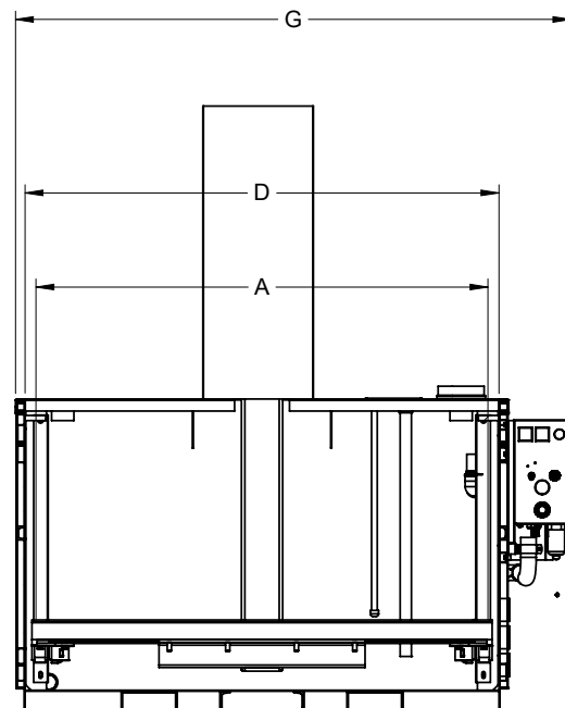
FRONT CROSS SECTION
